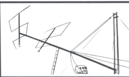
Antenna is then arranged and mounted on mast as a second step. All elements under 15' long are factory assembled, simplifying installation.
